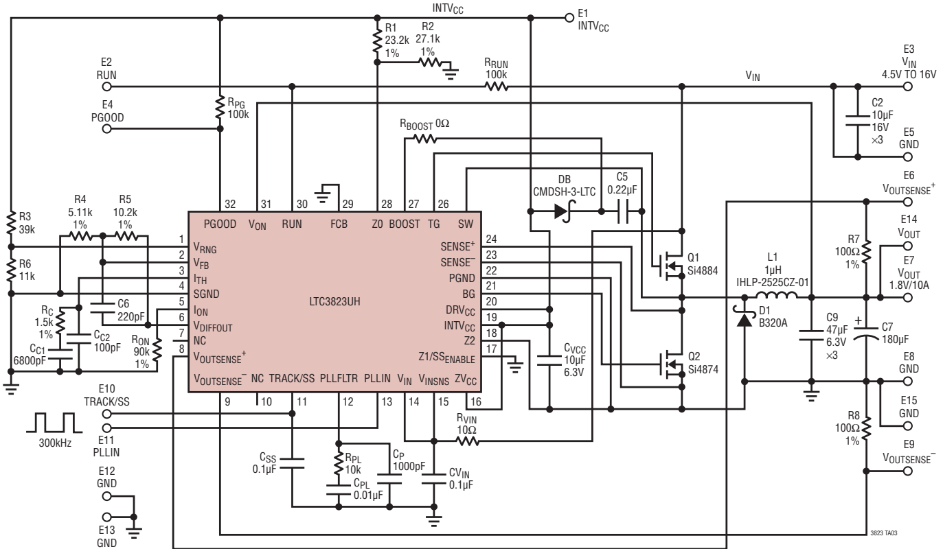
Design Example: 1.8V/10A with Synchronization
